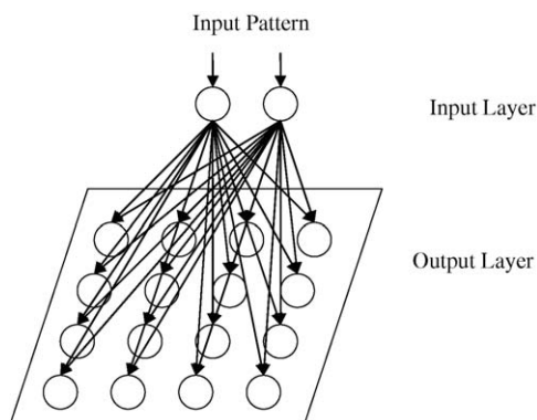
Fig. 1. The architecture of the SOM.
