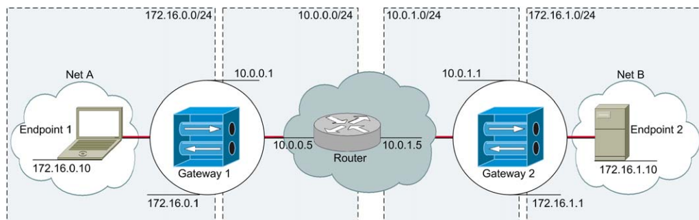
Fig. 2 – Laboratory layout.
