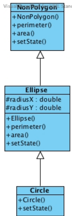
Figure 3: NonPolygon class hierarchy
