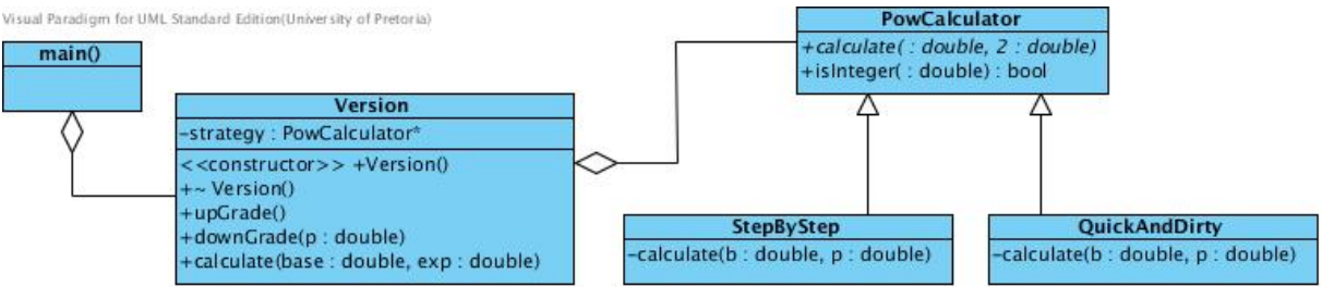
Figure 4: Class Diagram of a system illustrating the implementation of the Strategy design pattern
