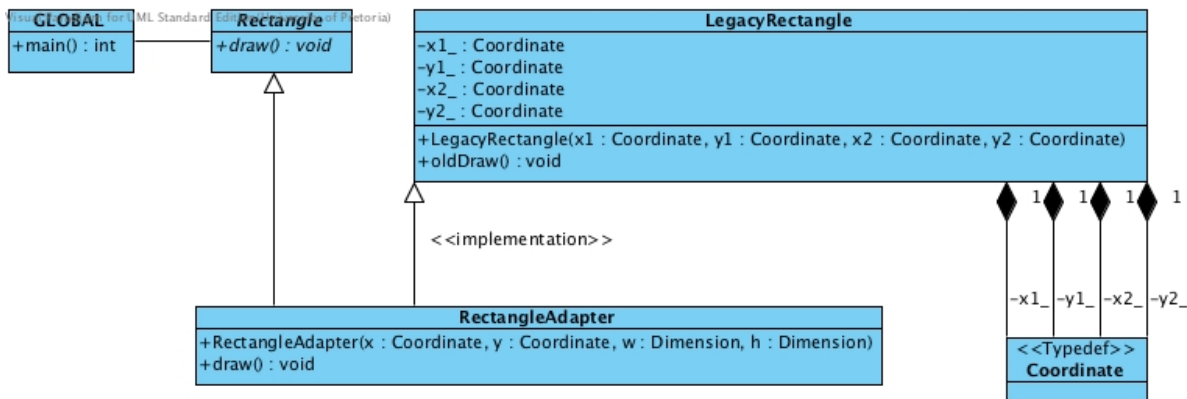
Figure 6: Rectangle example - class adapter
