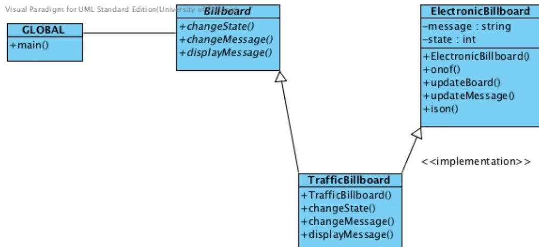
Figure 5: Billboard example - class adapter
