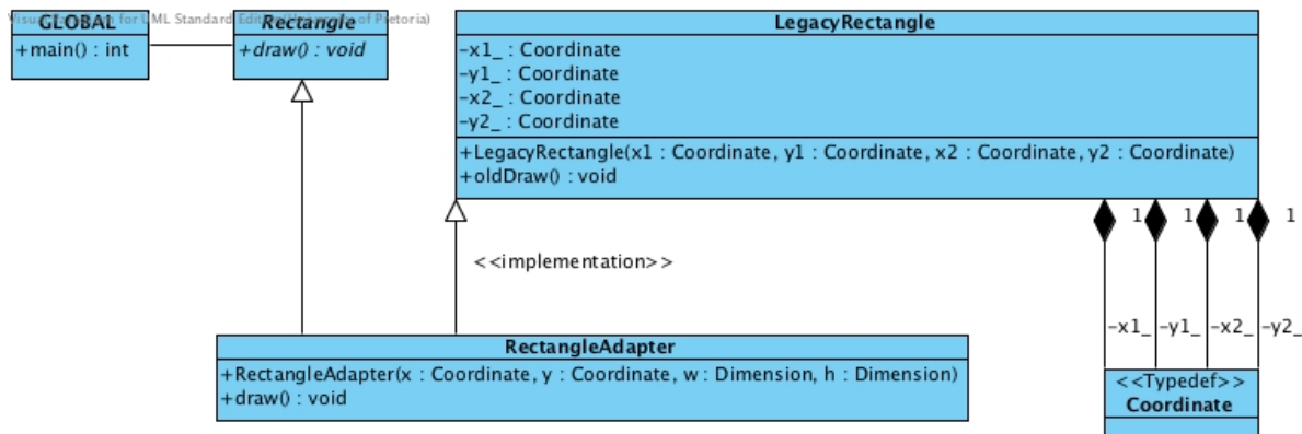
Figure 6: Rectangle example - class adapter
