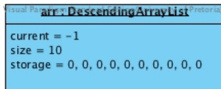
Figure 10: Object diagram on arr creation
