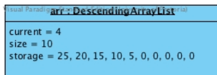
Figure 12: Object diagram after sorting
