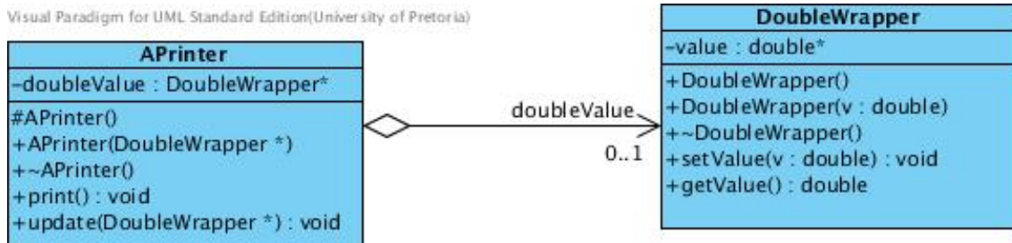
Figure 8: Aggregation association
