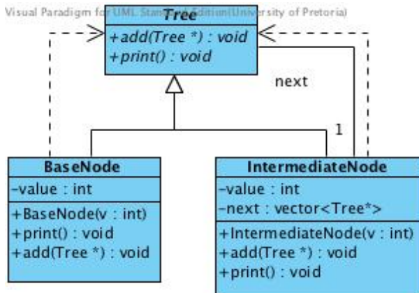
Figure 3: Tree example
